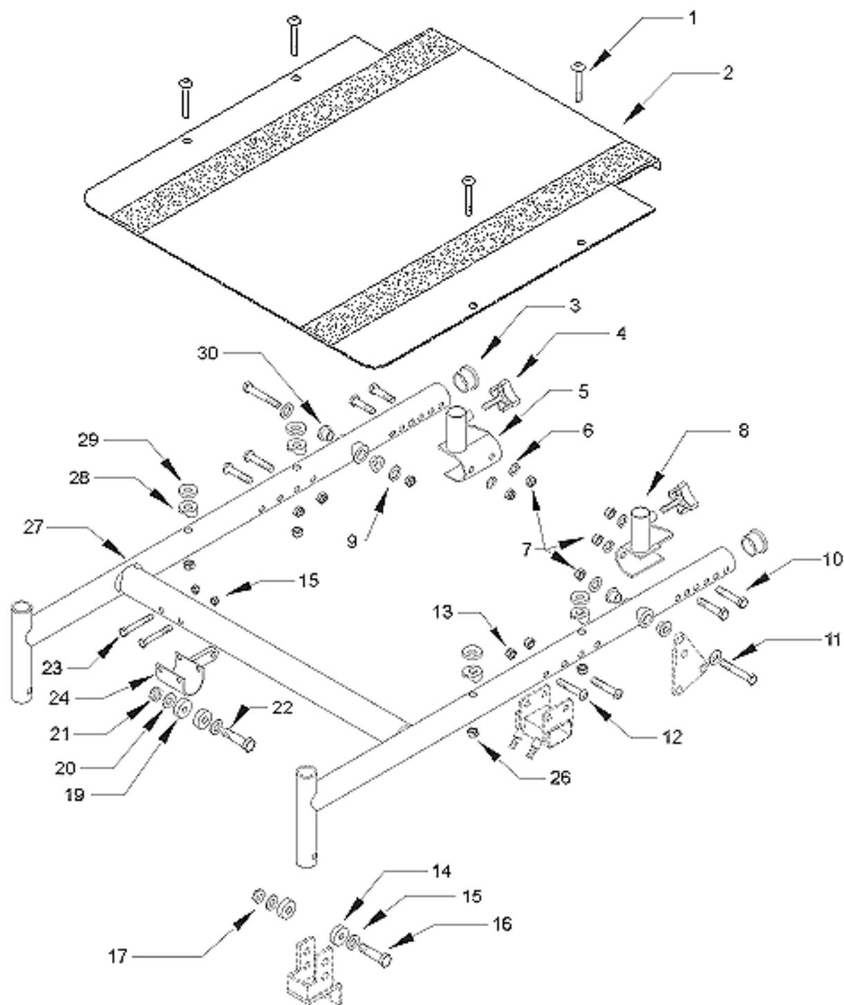
F55 seat frame MKI
