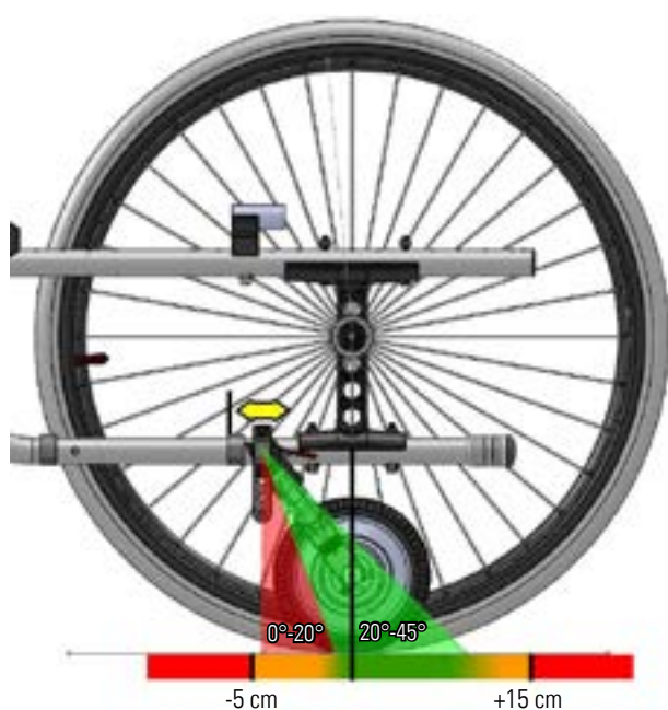
Assembly Breezy X-Family wheelchairs with Empulse R20
