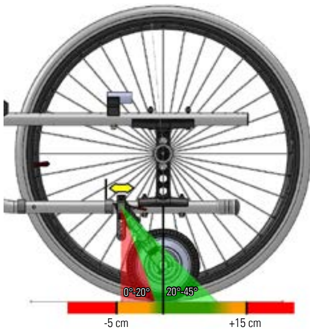
Assembly Breezy X-Family wheelchairs with Empulse R20
