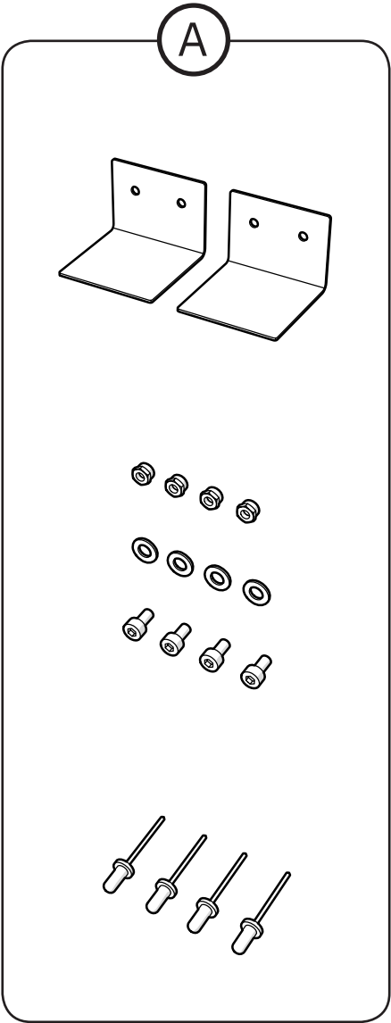
A 805073 Festebeslag for batterideksel kpl REAL 6100 PLUS Raising protection for battery cover Cpl REAL 6100 PLUS
