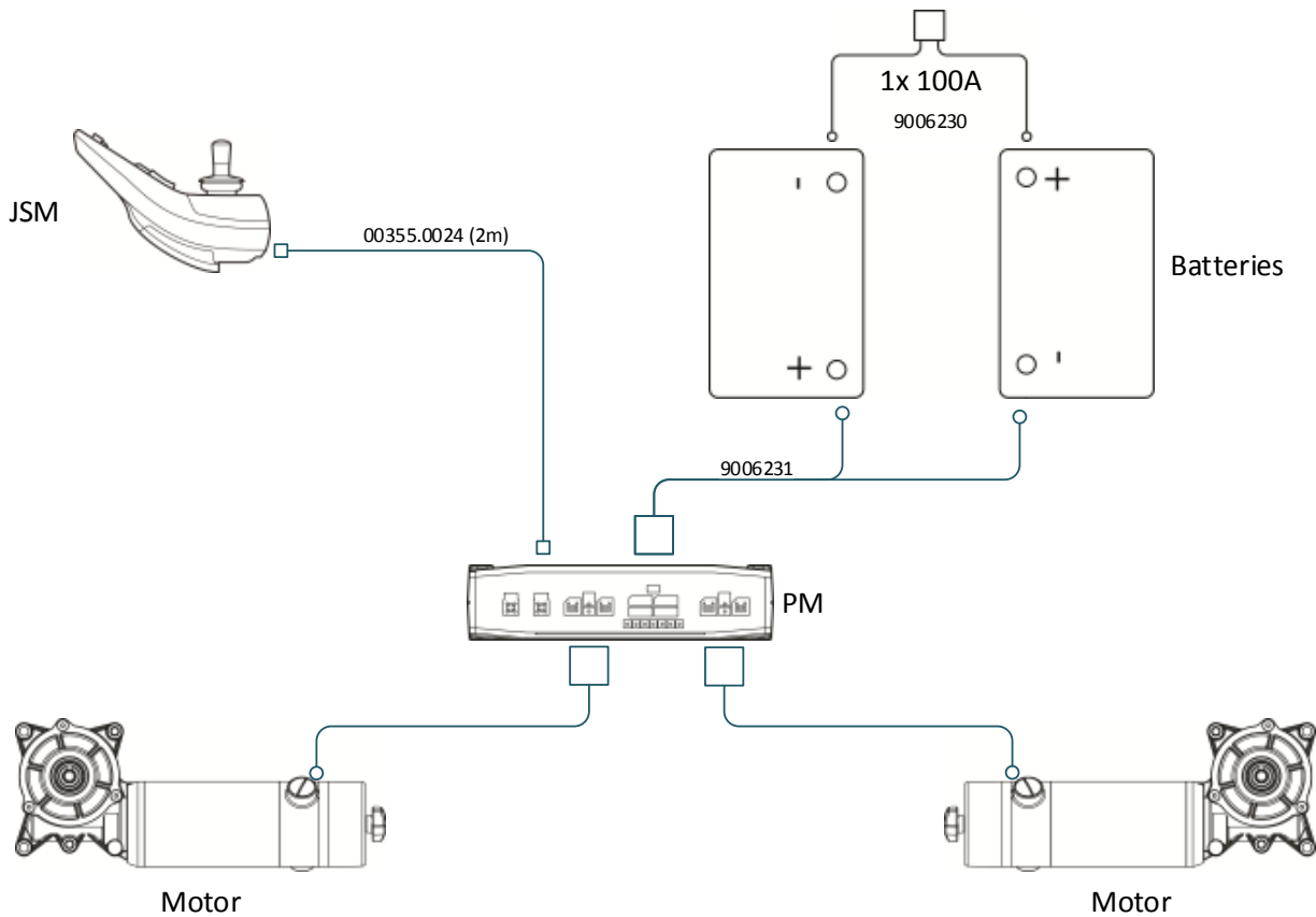
DX2 Battery & Motor connections (Drive only)
