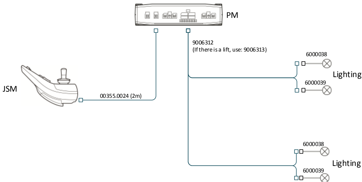
DX2 Drive & Lights
