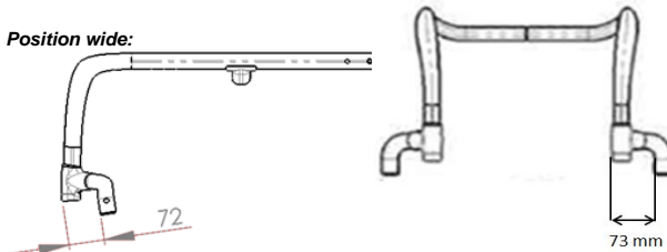
KRR040052 Single-post sideguard, armpad (33 cm)
