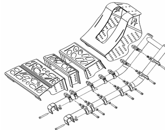
Performance Backrest
